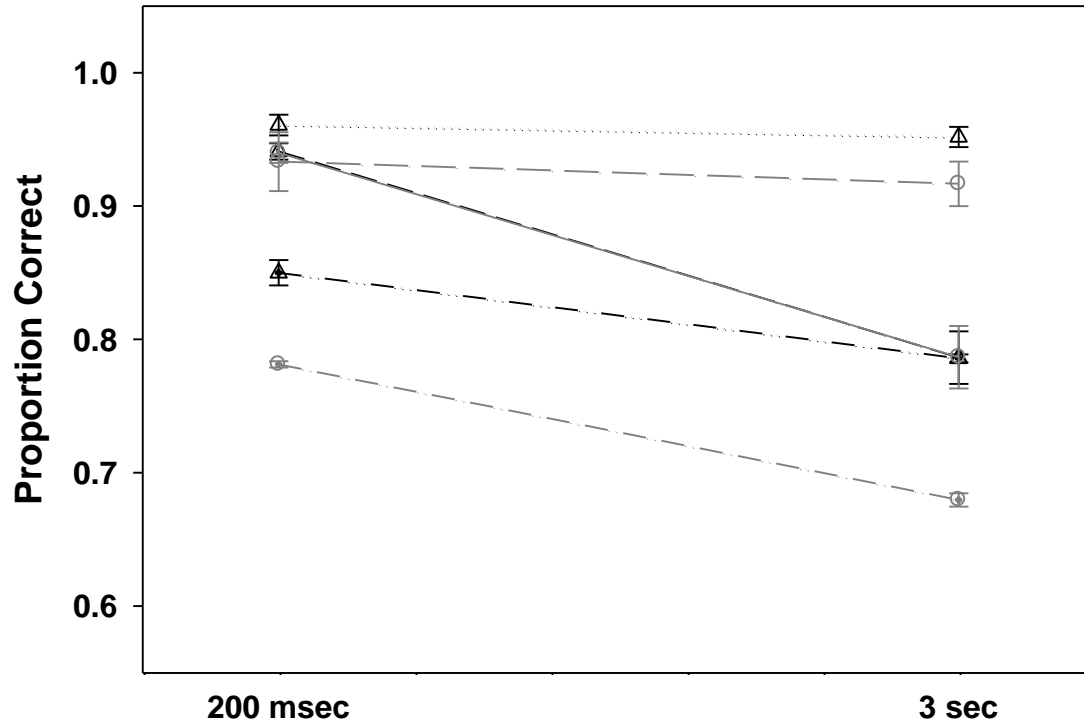
Figure 2. Mean Accuracy Scores in the 3 sec Delay Period as a Function of Perceptual Encoding at 200 ms: Good vs Poor Encoders
