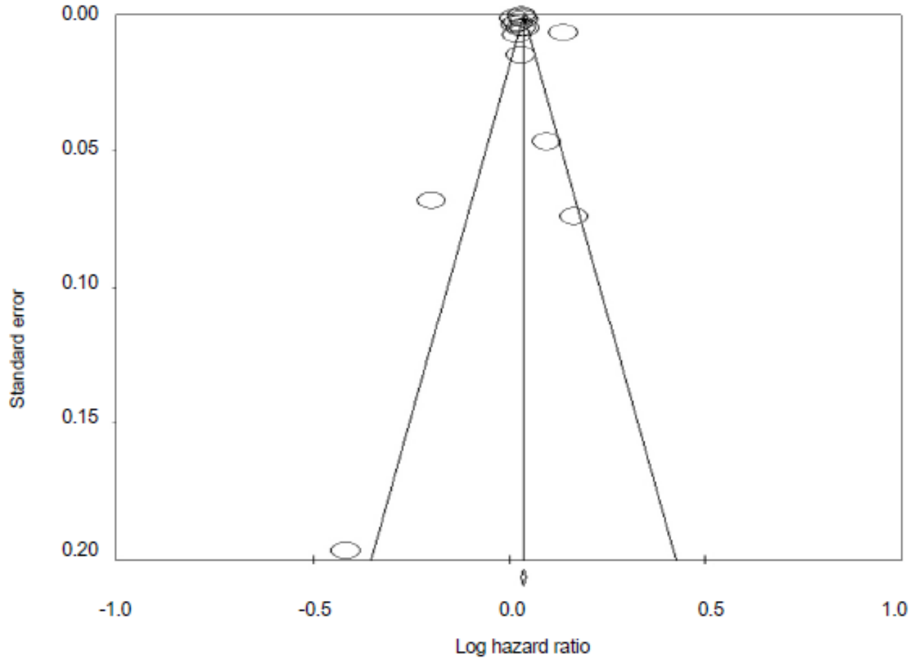
Figure S1. Funnel graph for the assessment of potential publication bias. The funnel graph plots the log adjusted hazard ratio against the standard error of the log adjusted hazard ratio. The dashed line indicates the 95% confidence interval of the log adjusted hazard ratio. The funnel plot shows approximate symmetry, and the result of the Egger test for publication bias is not significant ( P=0.74 ).
