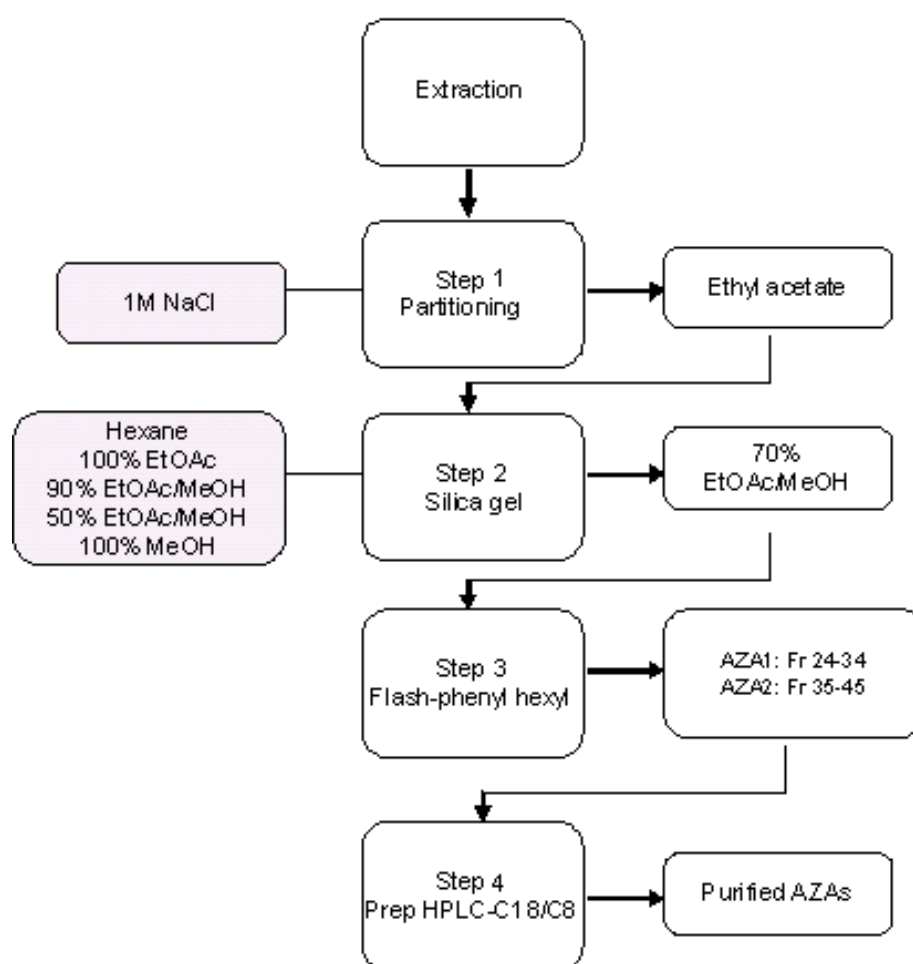
Figure S3. Procedure isolation of AZAs from A. spinosum .
