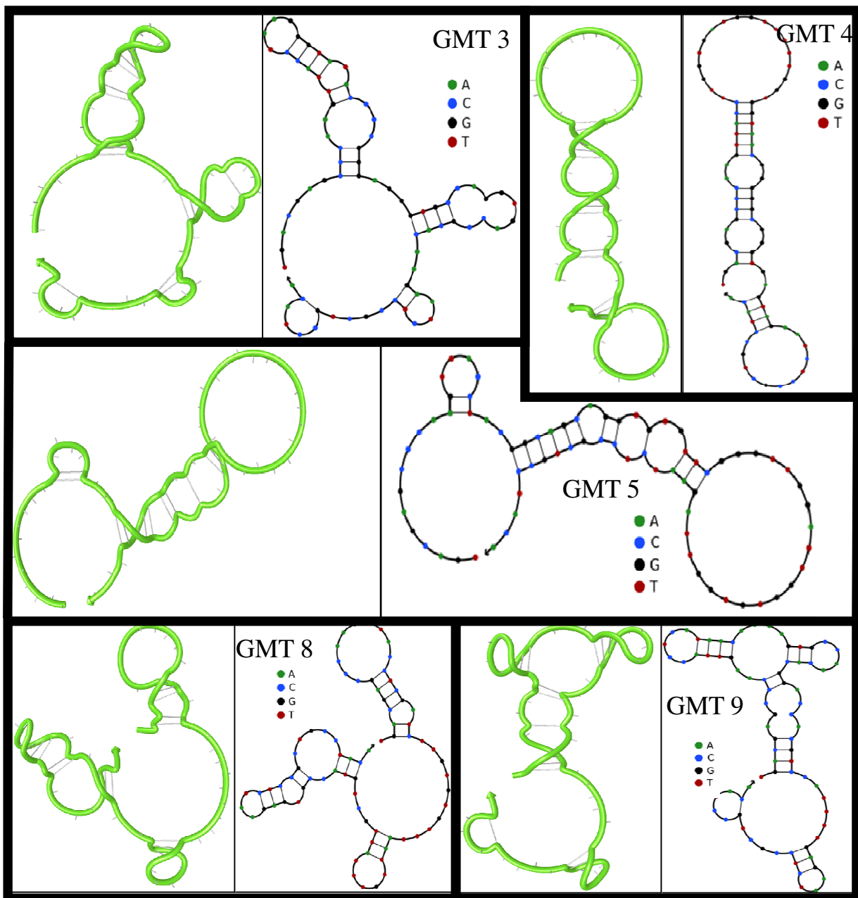
Figure S-1. Secondary structure analysis of selected aptamers.
