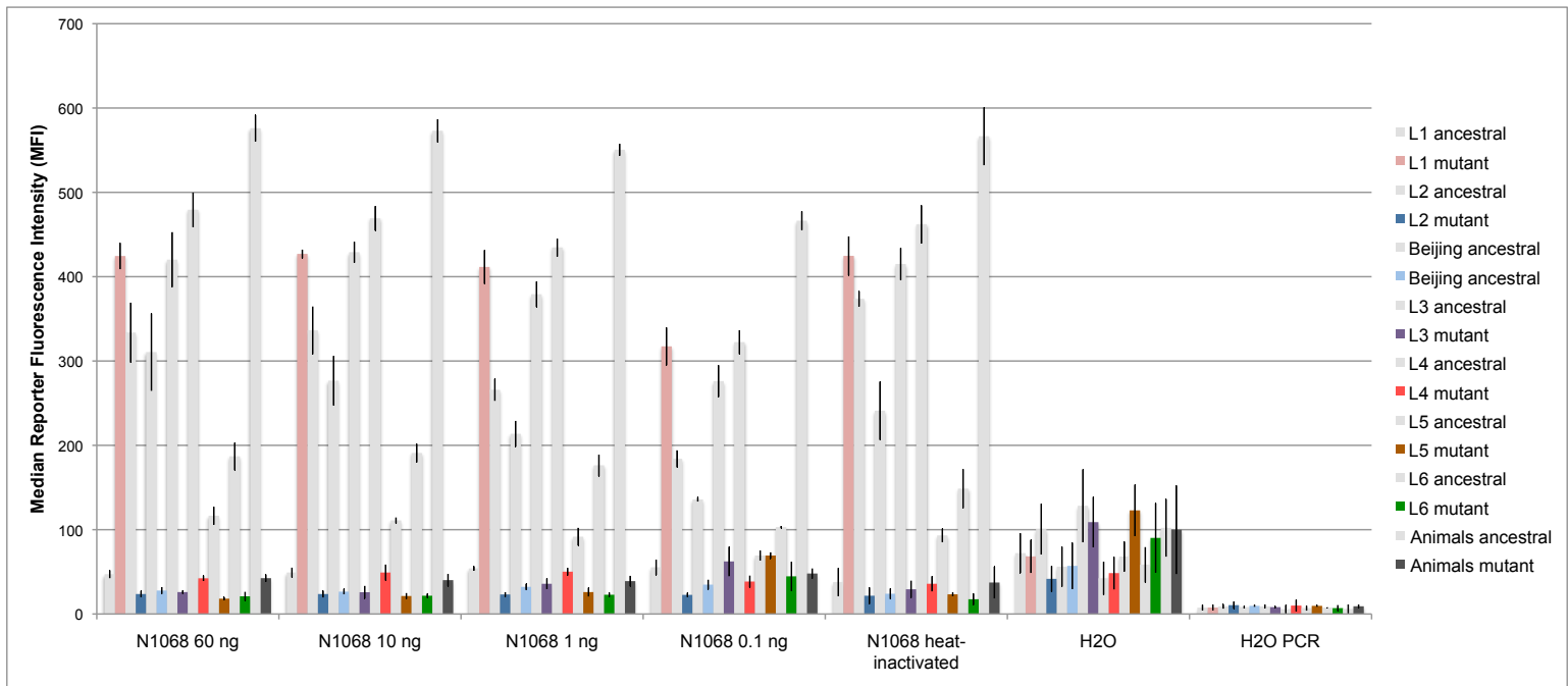
Figure S2. Dilution series of DNA from a clinical isolate of Lineage 1.
