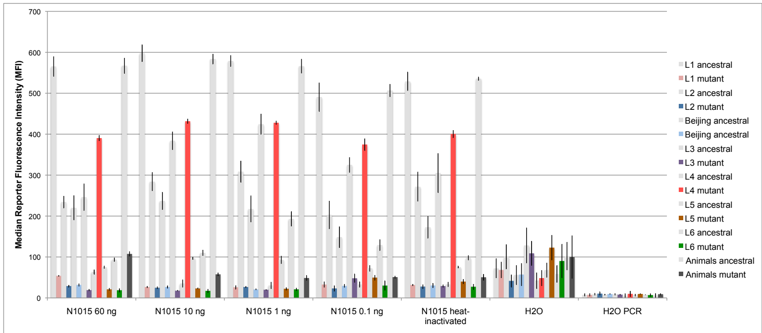
Figure S5. Dilution series of DNA from a clinical isolate of Lineage 4.
