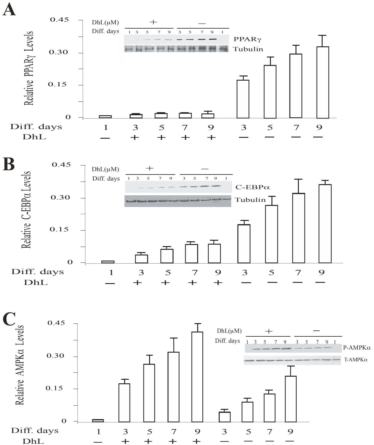
Supplementary Fig. 3. Dehydroleucodine selectively alters the expression of PPAR \gamma , C-EBP \alpha and AMPK \alpha . 3T3-L1 preadipocytes were induced to differentiate by induction media into adipocytes in the absence (insert: -DhL, control) or in the presence (insert: +DhL) of 8 \mu M DhL. Total protein extracts were prepared at day 1, 3, 5, 7 and 9 from each sample. The proteins were subset to 12% SDS-PAGE electrophoresis, blotted to a nitrocellulose membrane, and probed with anti-bodies specific to PPAR \gamma , C-EBP \alpha , AMPK \alpha and tubulin. Relative levels of proteins were determined by densitometry as describe in Material and Methods. Data represent the mean \pm S.E.M. of three independent experiments.
