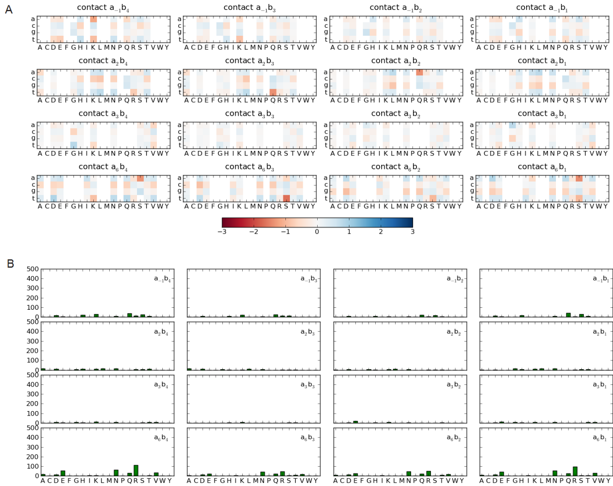
Figure S1. (A) Heat plot of log-odd scores for observed versus expected nucleotide frequencies in negative examples for each amino acid in each of the 16 contacts; (B) the corresponding \chi^2 values.
