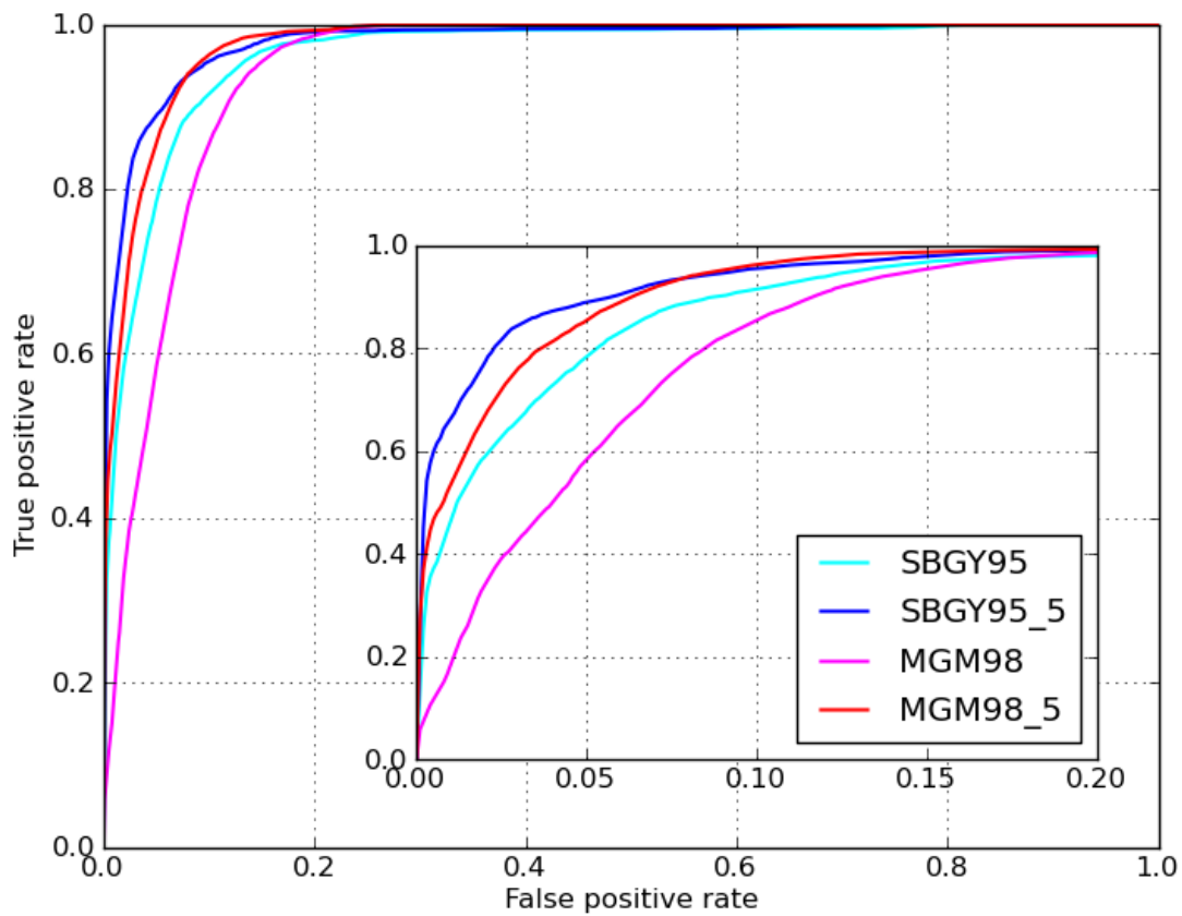
Figure S2. ROC curves for data used in cross-validation testing of non-SVM methods: SBGY95 based on the canonical model (cyan) and based on consensus 5-contact binding model (blue); MGM98 based on the canonical model (magenta) and based on consensus 5-contact binding model (red).
