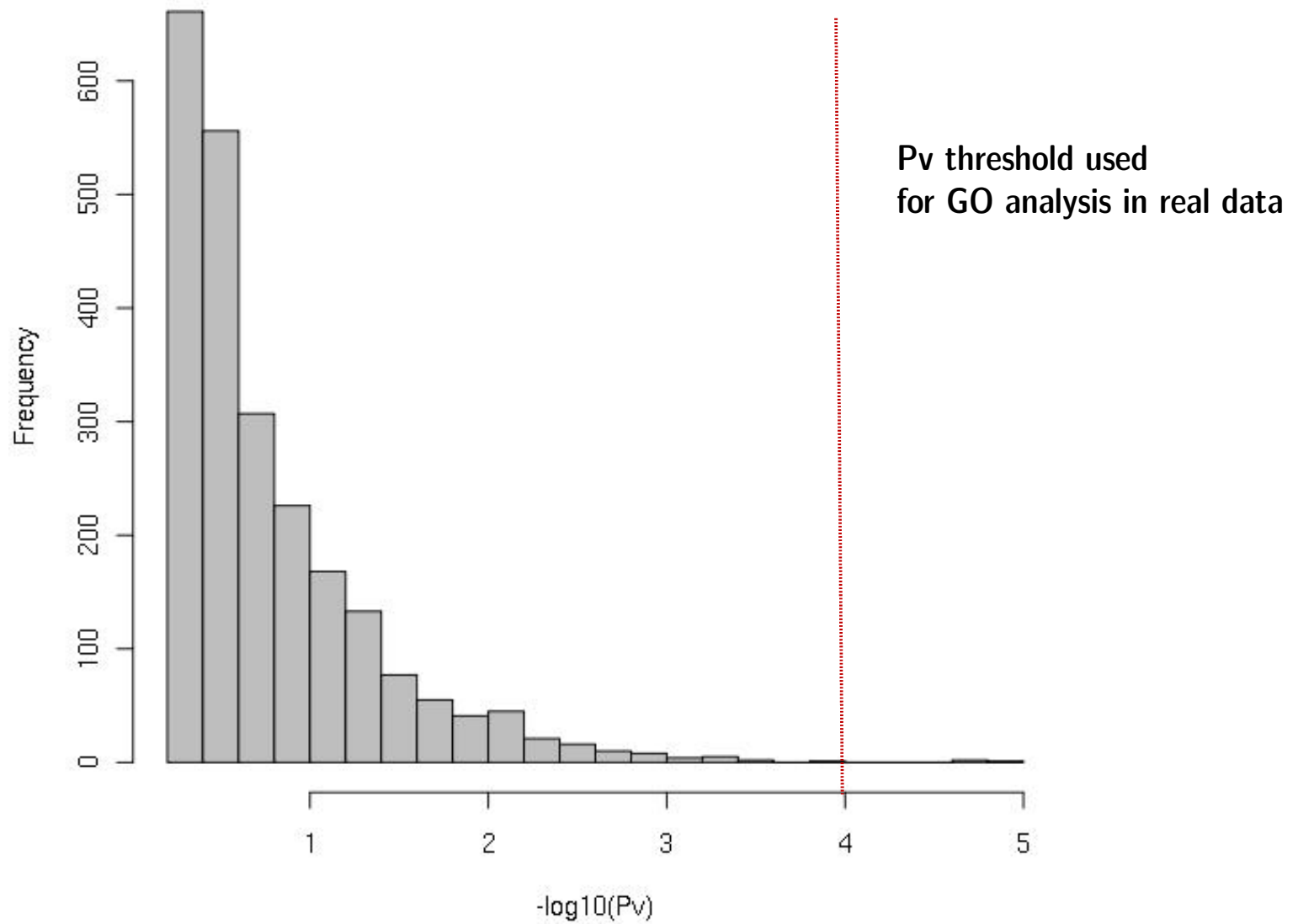
Supplementary Figure 2. GO enrichment p-value distribution in randomized target sets
