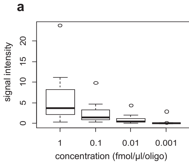
Additional file 5. Microarray signals of different concentrations of synthetic template oligos. (a) Boxplots showing the distribution of signals in each concentration and (b) line plots showing mean signals of individual probes.
