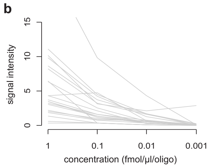
Additional file 5. Microarray signals of different concentrations of synthetic template oligos. (a) Boxplots showing the distribution of signals in each concentration and (b) line plots showing mean signals of individual probes.
