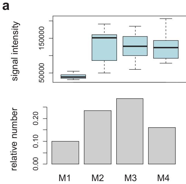
Additional file 6. Microarray signals of probes aligning with mismatches to full-length rRNA gene sequences present in the samples M1-4 (upper panels). In lower panels, relative 454 read numbers of corresponding sequences.
