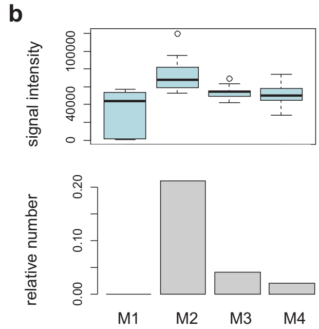
Additional file 6. Microarray signals of probes aligning with mismatches to full-length rRNA gene sequences present in the samples M1-4 (upper panels). In lower panels, relative 454 read numbers of corresponding sequences.
