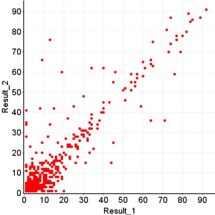
TBK1 inhibition by the LOPAC library
