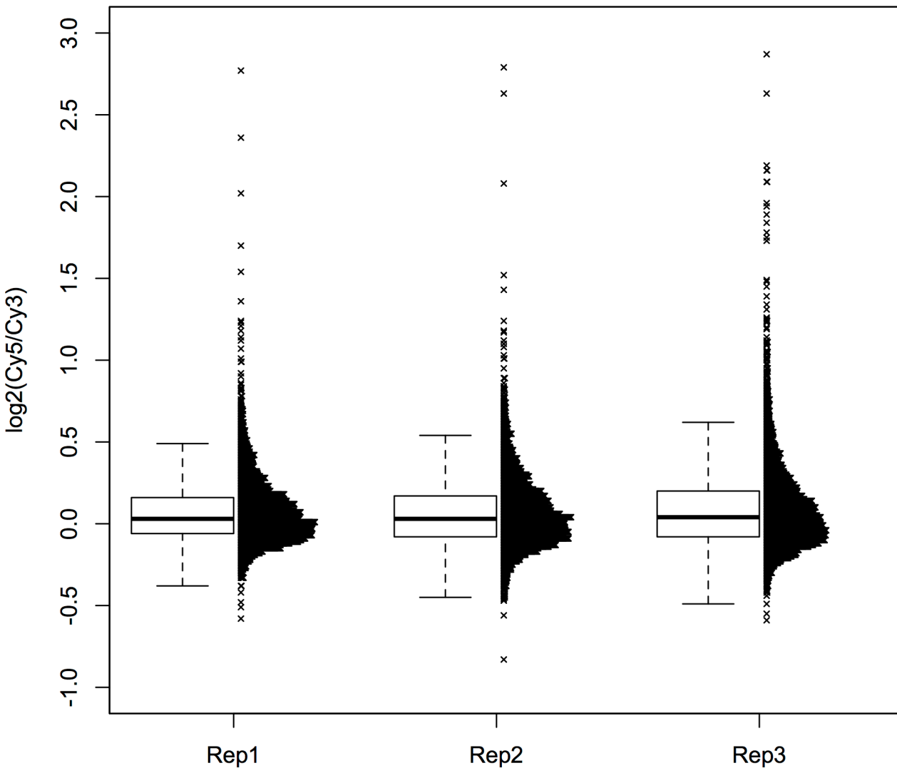
Log2(Cy5/Cy3) Ratio by Gene
