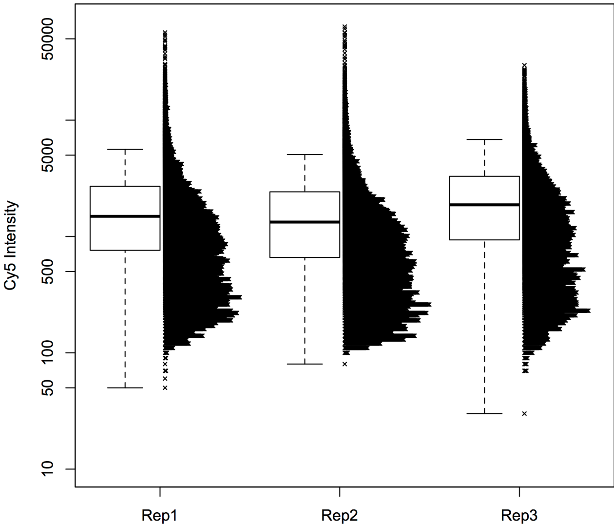
Cy5 Intensity by Probe
