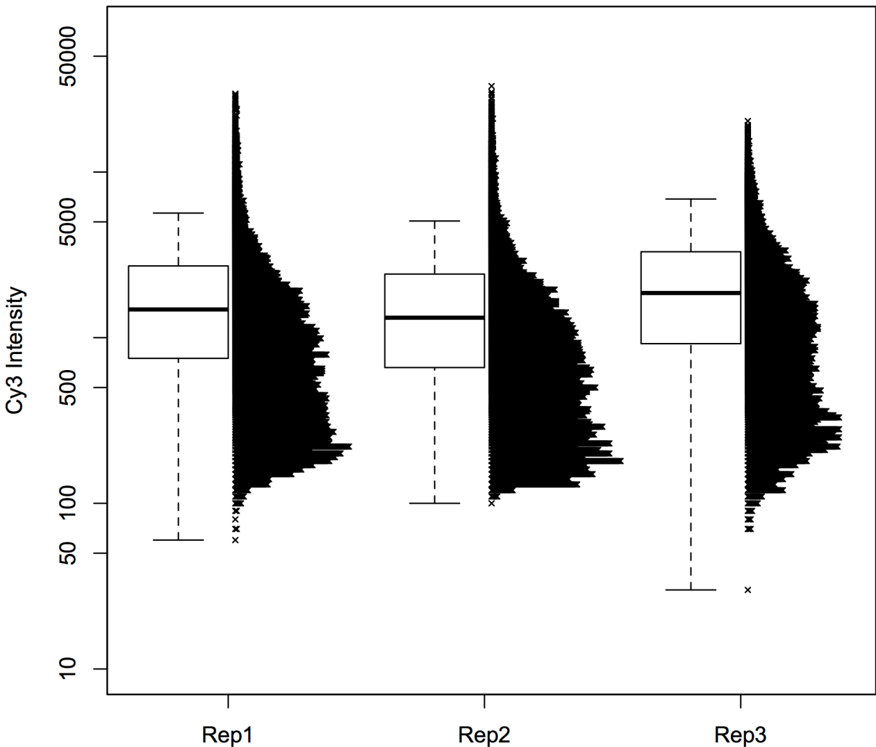
Cy3 Intensity by Probe
