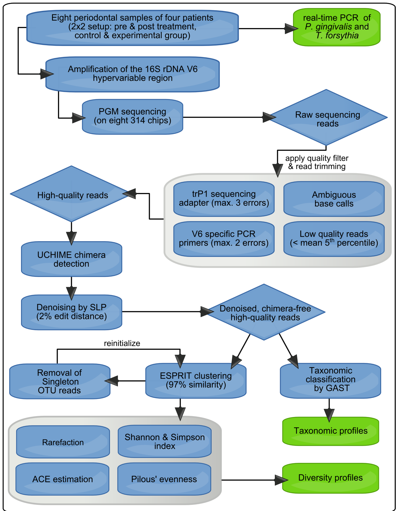
Figure S1. Schematic overview of the applied experimental and bioinformatic steps throughout the analysis. For a more detailed description of each individual step please see the Methods section.
