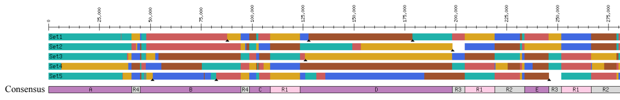
Figure S2. Comparison of the five mitochondrial genome assemblies from sequence sets 1-5. Different colors identify different contigs. Triangles indicate missing connections between contigs. Letters in the consensus sequence indicate single copy regions (A-E) and repeated regions (R1-R4).
