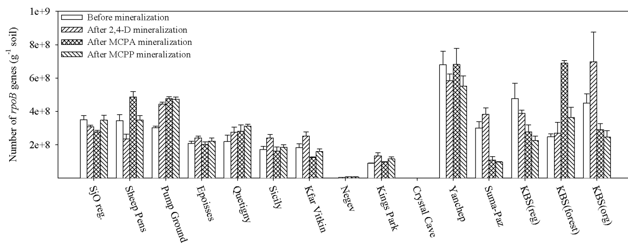
Figure S2. Quantification of rpoB genes. Error bars represent standard errors of the mean for soil triplicates.
