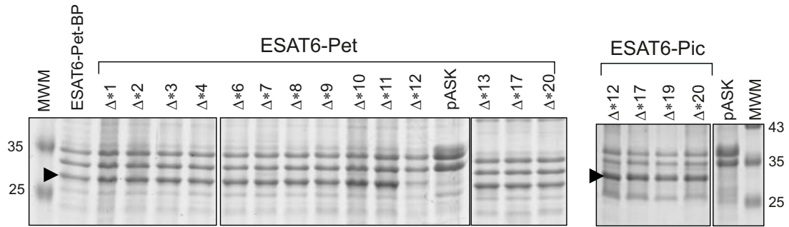
Figure S5. Identification of minimal AT module permitting secretion of heterologous proteins to the culture supernatant fraction. SDS-PAGE analyses of the OM fractions corresponding to some culture supernatant fractions depicted in Figure 3 are shown. The presence in the OM of the cleaved Pet and Pic \beta -barrel domains is indicated with an arrow. The size of molecular weight markers (MWM, kDa) is indicated.
