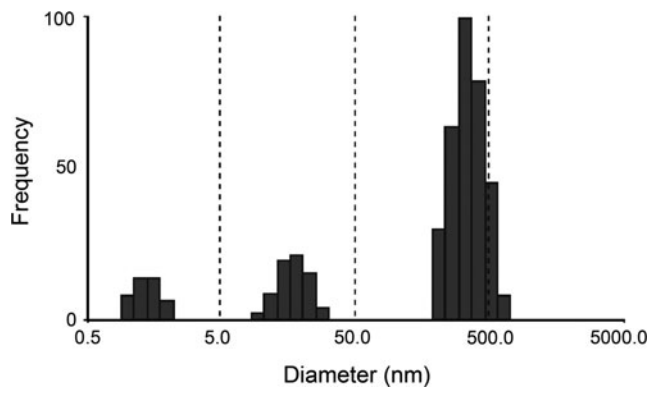
SUPPLEMENTARY FIG. S1. Representative dynamic light-scattering data for PDMS particles in an aqueous solution. PDMS, poly(dimethylsiloxane).
