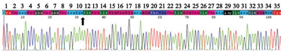
SUPPLEMENTARY FIG. S2. Electropherogram of a sequencing reaction from the V3 region of isolate 0008SP. The black arrow shows the observed deletion at position 11.
