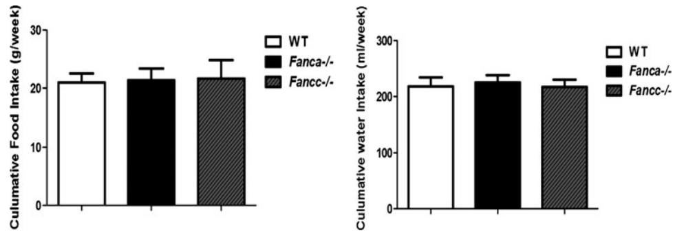
SUPPLEMENTARY FIG. S2. Food/water intake in mice. Fanca -/- or Fancc -/- mice and their wt littermates (6–8 weeks old) were divided into three to four mice per cage, and cumulative food ( left ) or water ( right ) intake was measured as described in Experimental procedures. Values are expressed as means±SD. FANCC, Fanconi anemia complementation group C; WT, wild-type.
