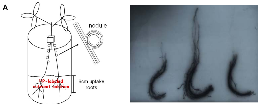
Figure S5. In situ assays for [ 33 P] Pi uptake using transgenic composite soybean plants. A, Graphical representation of the soybean roots treated in the [ 33 P] Pi solution. The bottom 6 cm of root regions were directly immersed in the 33 P labeled nutrient solution. Arrows indicated that the nodules in the upper roots were not exposed to the 33 P labeled nutrient solution. B, Autoradiograph of [ 33 P] Pi taken up by the bottom 6cm root regions.
