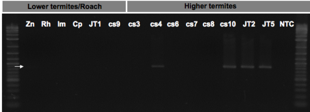
Figure S3. Products from nested PCR reactions using (i) universal fdhF primers followed by (ii) Amitermes-Gnathamitermes-Rhychoitermes clade specific primers on gut templates. NEB 2 log ladder was used. See Fig. S1 for template designations. Slight band in lane Zn was observed inconsistently and infrequently and is attributed to contamination during nested PCR.
