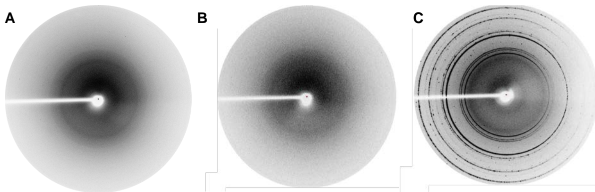
Supplemental Figure S2. X-ray diffraction of p53C aggregates obtained by high temperature. (A) WT p53C at pH 7.2; (B) R248Q p53C at pH 7.2 and (C) WT p53C at pH 5.0 were diffracted showing reflections from 4.7 to 10 Å, characterizing structures in cross \beta -sheets.
