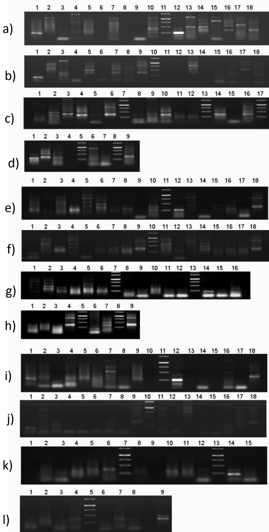
Figure S7(iii). 3C analysis of histone gene cluster during T-cell development.
