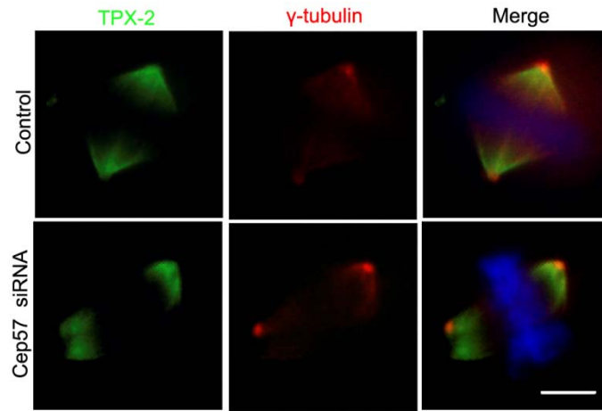
Figure S5 Control siRNA and Cep57 siRNA treated cells were stained for TPX-2 (green), \gamma -tubulin (red) and DNA (blue). Bar, 5 \mu m.
