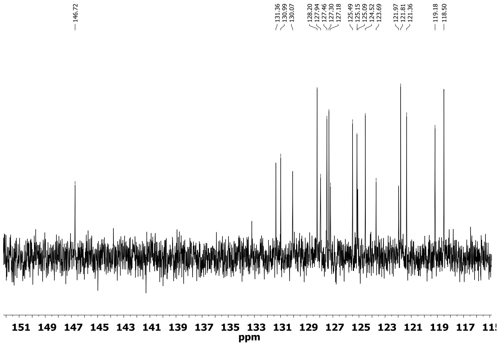
Figure S1. ^{13}\text{C} NMR spectra of 8-hydroxy-B[a]P-7-O-sulfate (M1)
