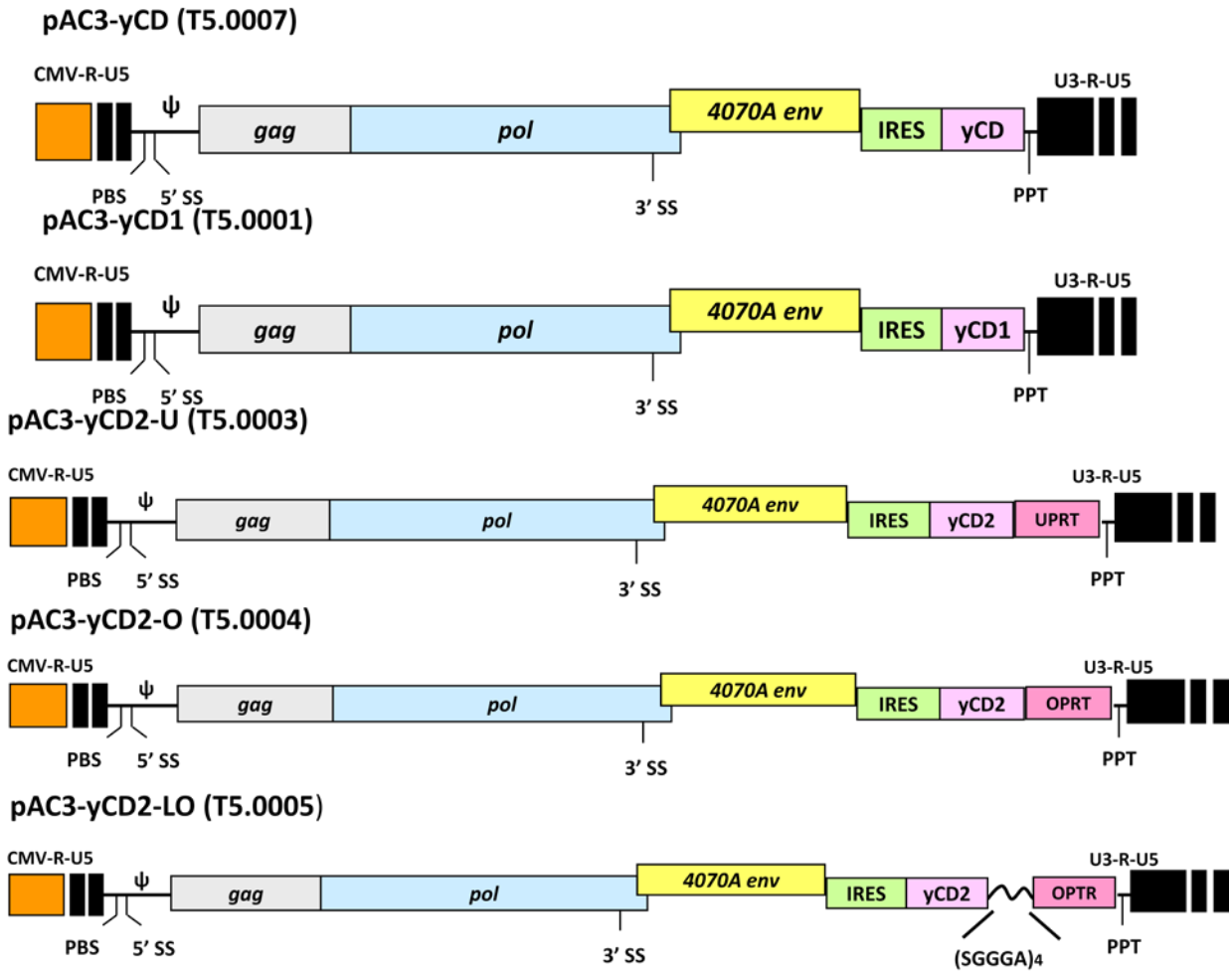
Supplemental Figure 1. Configuration of plasmid constructs encoding RRV's constructed from Moloney MLV with an amphotropic envelope and various CD and Hybrid CD genes. Names of the vectors are as shown and correspond to vectors in Table 1 in the main text.
