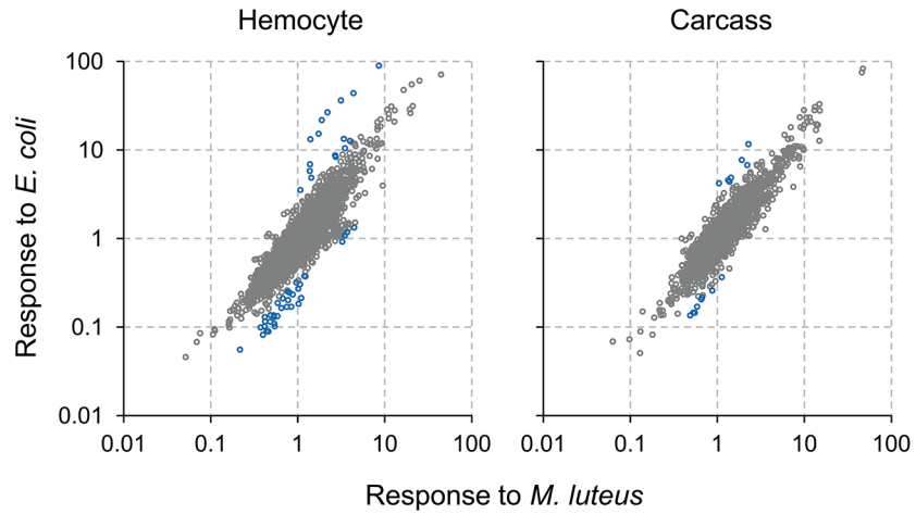
Fig. S4. Aedes aegypti hemocyte and carcass response to Escherichia coli - and Micrococcus luteus -challenge. The axes indicate expression ratios. Transcripts displaying a differential response to E. coli - relative to M. luteus -challenge are colored blue ( P < 0.01 and fold difference > 3 ).
