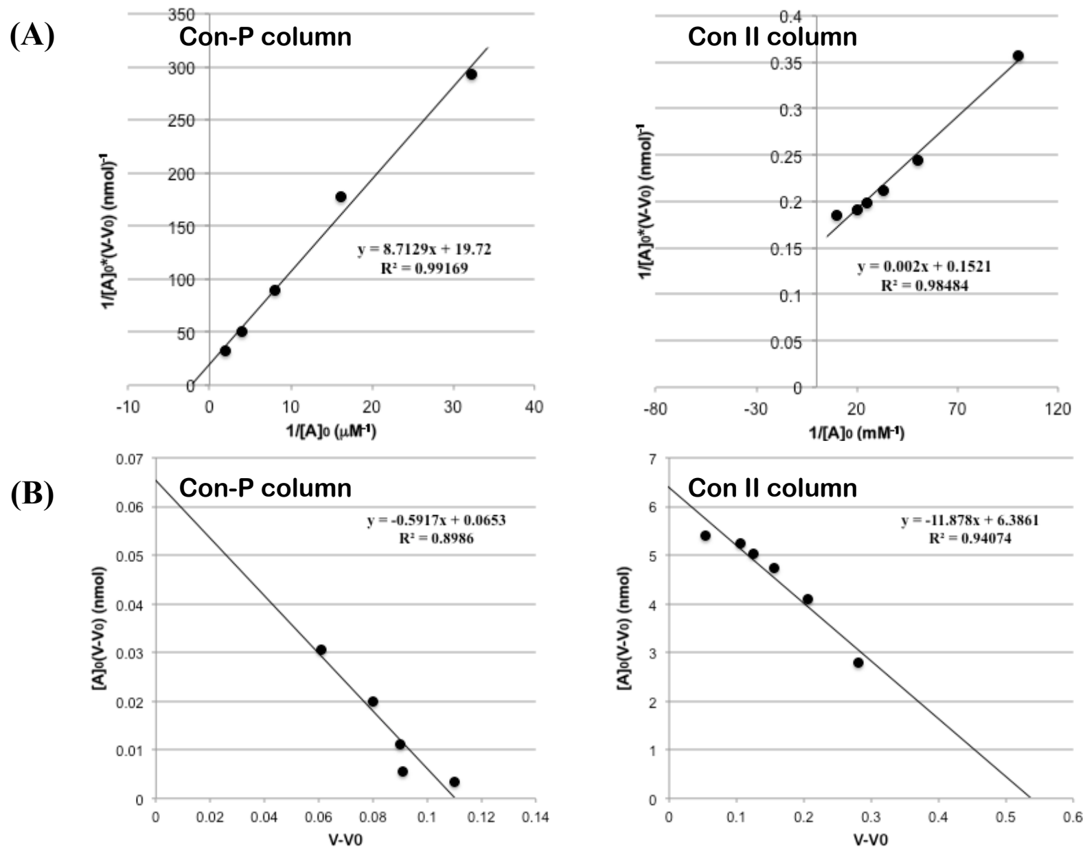
FIGURE S7. Determination of the column binding capacity ( Bt ) for Con-P conjugated (Con-P) and Con II conjugated (Con II) columns by Lineweaver-Burk plots (A) and Woolfe-Hofstee-type plots (B).
