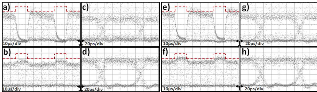
Supplementary Fig. S1: Data injection. Modulation with 15 μs electrical rectangular pulses at 20KHz repetition rate for 10Gb/s (a) data trace at the CROSS port (channel 3), (b) data trace at the BAR port (channel 3), (c) eye diagram at the CROSS port (channel 3), (d) eye diagram at the BAR port (channel 3), (e) data trace at the CROSS port (channel 4), (f) data trace at the BAR port (channel 4), (g) eye diagram at the CROSS port (channel 4), (h) eye diagram at the BAR port (channel 4).
