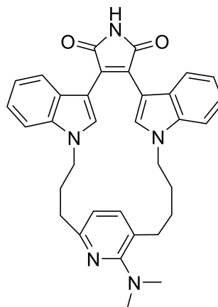
ID: 50 Name: Jonjon-1 PDB ID: 2OW3
