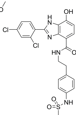
ID: 37 Name: Benzoimidazole-1 PDB ID: 2O5K
