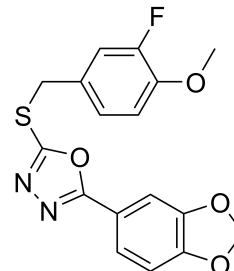
ID: 98 Name: OxaD-0 PDB ID: 3F7Z
