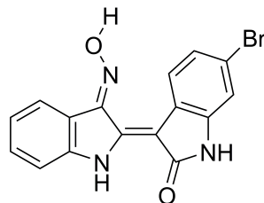
ID: 60 Name: LM-5 PDB ID: 1UV5
