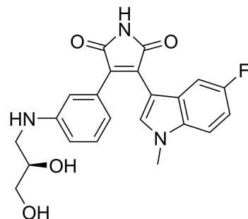
ID: 97 Name: Maleimide PDB ID: 1R0E
