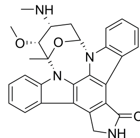
ID: 199 Name: Staurosporine PDB ID: 1Q3D
