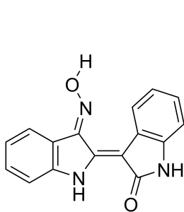
ID: 77 Name: LM-29 PDB ID: 1Q41
