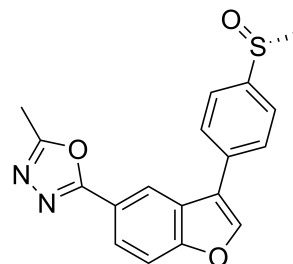
ID: 99 Name: OxaD-00 PDB ID: 3GB2
