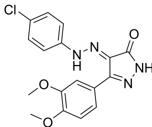
ID: 153 Name: Pyzo-11 PDB ID: 3L1S
