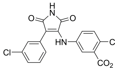
ID: 198 Name: RM-0 PDB ID: 1Q4L
