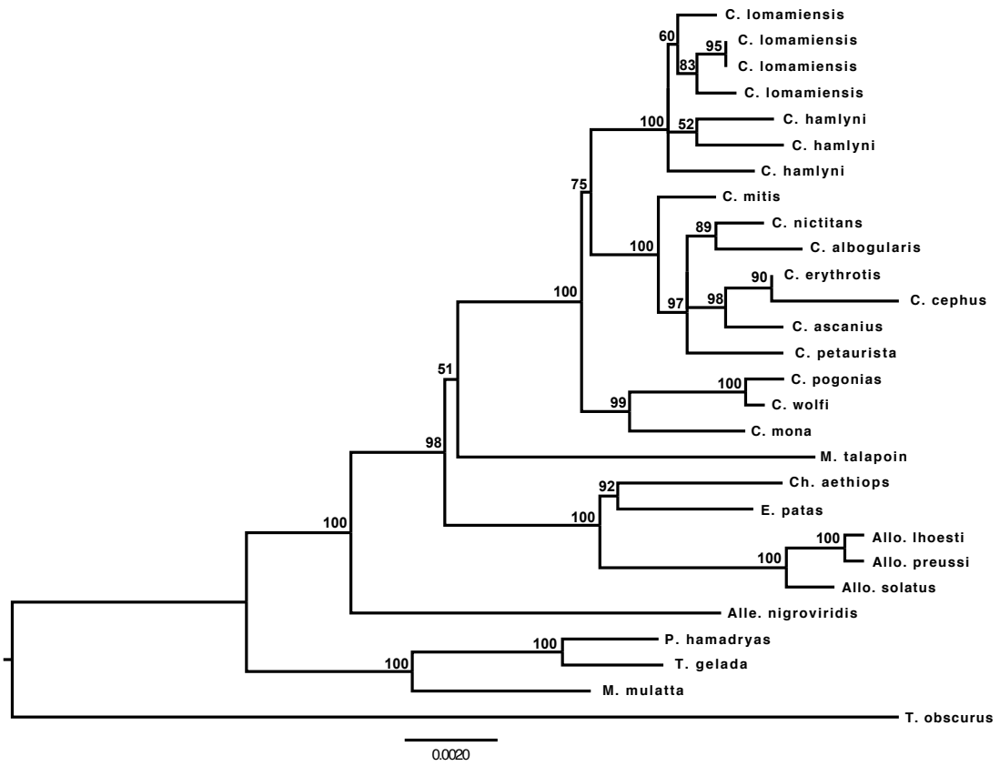
Fig. S3. Maximum likelihood tree, Xq13.3 homolog. The scale at the bottom is in units of nucleotide substitutions per site.
