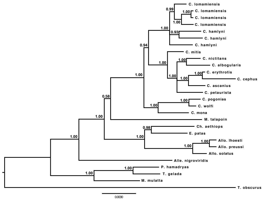
Fig. S4. Bayesian tree, Xq13.3 homolog. The scale at the bottom is in units of nucleotide substitutions per site.
