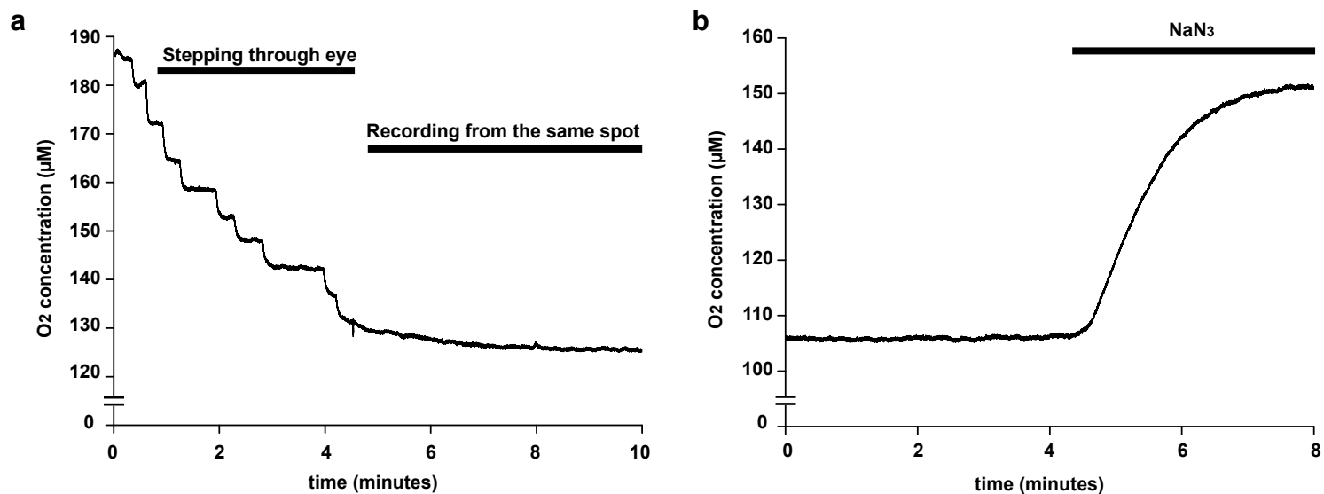
Supplementary Figure 4. (a) Variation in [O 2 ] as the electrode is pushed deeper in the retina in steps. (b) Increase in [O 2 ] deep in the tissue after addition of NaN 3 in the bath.
