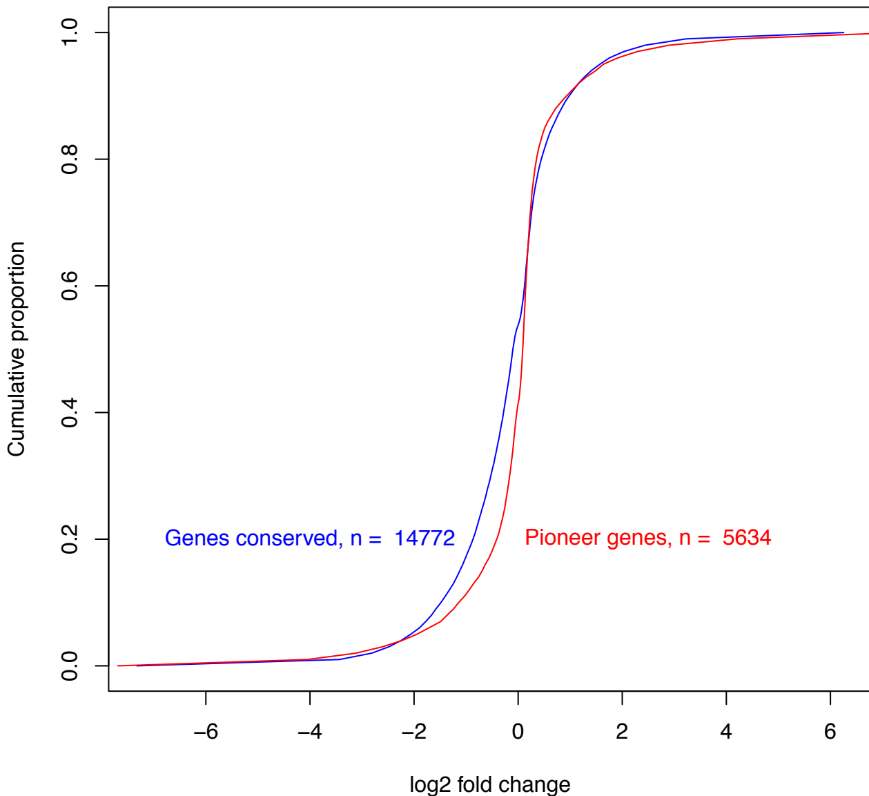
Cumulative distribution of fold changes of P. pacificus pioneer genes, and P. pacificus genes with orthologs. KS test p-value < 2E-16
