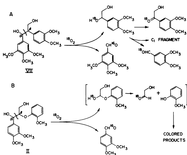
FIG. 5. Scheme showing ligninase action on \beta -1 (A) and \beta -O-4 models (B). \beta -1 and \beta -O-4 models are represented by VII and II, respectively. Compounds in brackets (B) have been deduced from studies with three \beta -O-4 models (see text). Incorporation of ^{18}O from ^{18}O_2 into the C_\beta -derived product (III) from model VII is established. Similar incorporation of ^{18}O is presumed in the case of model II, as shown.
