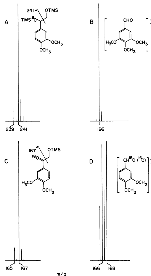
FIG. 6. Diagnostic portions of mass spectra of products formed on enzymatic oxidation of model VII. The reaction was under ^{18}O_2 and with H_2^{16}O_2 . The major fragments from the trimethylsilyl (TMS) derivatives are shown for products III (A) and IV (C). The molecular ion regions are shown for 3,4,5-trimethoxybenzaldehyde (B) and veratraldehyde (D). Regions shown contain the base peaks (100%, >3600 ion counts). Molecular ions were present for the trimethylsilyl derivatives of compounds III and IV at m/z = 344 (1.3%) and 270 (10.6%), respectively.
