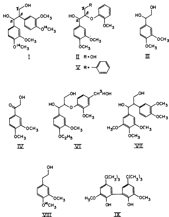
FIG. 1. Molecular formulae.
