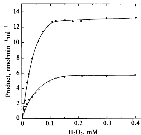
FIG. 4. Effect of H_2O_2 on enzyme activity. H_2O_2 was added to reaction mixtures containing enzyme at 5 \mu g/ml , 0.1% Tween 80, 0.1 M sodium tartrate at pH 3.0, and 0.4 \text{ mM} veratryl alcohol ( \bullet ) or 1.15 \text{ mM} model II ( \circ ). The formation of veratraldehyde from veratryl alcohol and the formation of aryl-conjugated carbonyl from model II was monitored by the associated increase in absorbance at 310 nm.
