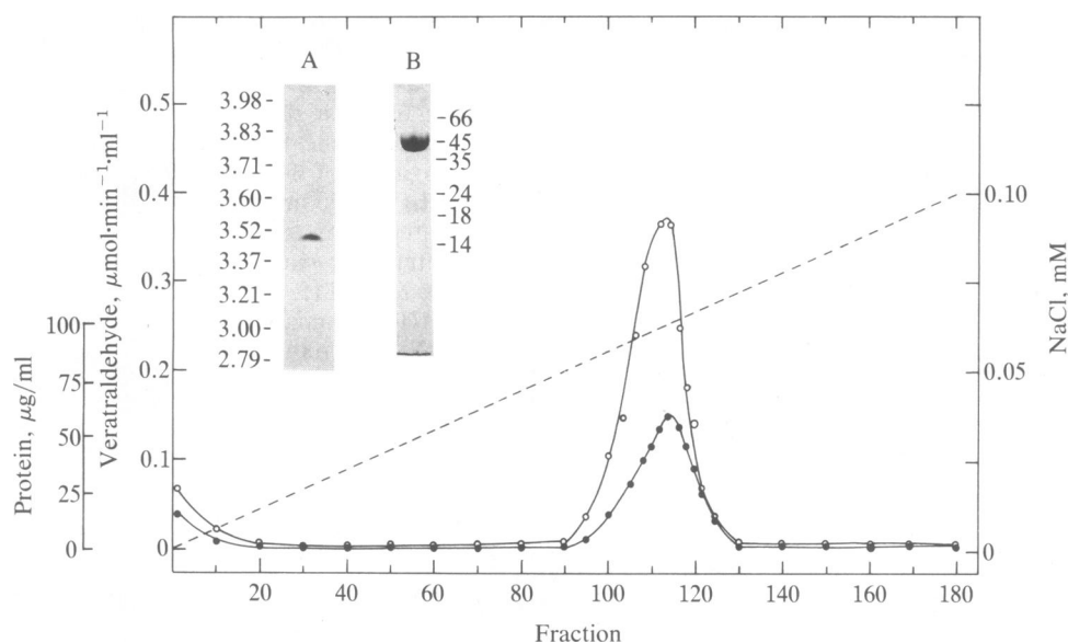
FIG. 2. Elution profile of the ligninase enzyme from a column of DEAE-Bio-Gel A. Fractions (2.2 ml) were assayed for H_2O_2 -requiring activity for the oxidation of veratryl alcohol ( \circ ) and for protein content ( \bullet ). Purity is assessed by isoelectric focusing (Inset A) and NaDodSO_4 /polyacrylamide gel electrophoresis (Inset B). Numbers adjacent to gel A are pH values and numbers adjacent to B are M_r \times 10^{-3} .
