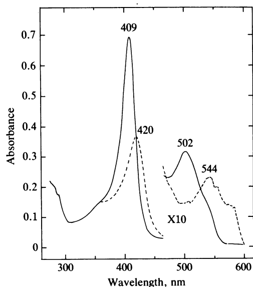
FIG. 3. Absorption spectrum of ligninolytic enzyme. The spectrum of the purified enzyme ( 0.3 \text{ mg/ml} in 5 \text{ mM} sodium tartrate, pH 4.5) was recorded in the presence (---) and absence (—) of 21 \mu M H_2O_2 . Numbers above peaks denote wavelength maxima.
