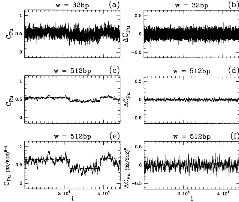
Figure 4. Fluctuations of the purine content within non overlapping boxes (Figure 6(a)) of size w as a function of the box position i for the DNA sequence of the bacteriophage \lambda ( L = 48502 bp): (a) C_{Pu} for w = 32 bp; (c) C_{Pu} for w = 512 bp and (e) C_{Pu} for w = 512 bp after being rescaled according to equation (2) with H = 0.6 . Fluctuations of the corresponding wavelet coefficients as computed with the Haar wavelet (Figure 6(b)): (b) \Delta C_{Pu} for w = 32 bp; (d) \Delta C_{Pu} for w = 512 bp and (f) \Delta C_{Pu} for w = 512 bp after being rescaled according to equation (8) with H = 0.5 . In (c) and (e) the horizontal dashed segments correspond to the patches of different average purine concentrations.
