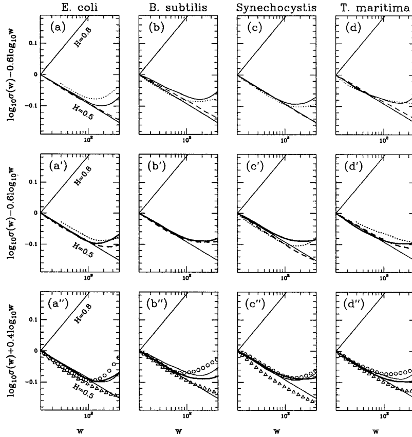
Figure 11. Global estimate of the r.m.s. of WT coefficients of Escherichia coli (a-a''), Bacillus subtilis (b-b''), Synechocystis sp. PCC 6803 (c-c'') and Thermotoga maritima (d-d''): \log_{10} \sigma_{WT}(w) - 0.6 \log_{10} w is plotted versus \log_{10} w . The analyzing wavelet is the first-derivative of the Gaussian function g^{(1)} (Figure 6(d)). The various curves correspond to the same mono-, di- and tri-nucleotide coding rules as in Figure 10.
