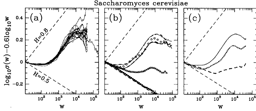
Figure 9. Global estimate of the r.m.s. of WT coefficients of the 16 chromosomes of S. cerevisiae : \log_{10} \sigma_{WT}(w) - 0.6 \log_{10} w is plotted versus \log_{10} w . The analyzing wavelet is the first-derivative of the Gaussian function g^{(1)} (Figure 6(d)). (a) Comparative analysis of the 16 chromosomes when using the 'A' mononucleotide coding. (b) Comparative analysis of the 'A' (grey solid line), 'T' (grey dashed line), 'G' (black solid line) and 'C' (black dashed line) mononucleotide codings with the 'Pnuc' (circles) and 'DNase' (triangles) trinucleotide codings; the black dots correspond to a randomly shuffled Pnuc table (see text). (c) Comparative analysis of the 'A' (+ 'T') mononucleotide coding (solid line) with the 'AA' (= 'TT') dinucleotide coding (dotted line) and the ' A_{iso} ' (= ' T_{iso} ') mononucleotide coding (dashed line). In (b) and (c), the results correspond to averaging over the 16 chromosomes. For coding rules see Materials and Methods.
