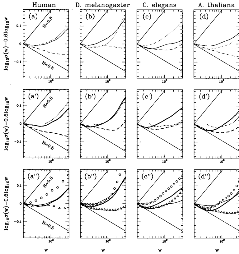
Figure 10. Global estimate of the r.m.s. of WT coefficients of the human chromosome 21 (a-a''), Drosophila melanogaster (b-b''), Caenorhabditis elegans (c-c'') and Arabidopsis thaliana (d-d'') genomes: \log_{10} \sigma_{WT}(w) - 0.6 \log_{10} w is plotted versus \log_{10} w . The analyzing wavelet is the first-derivative of the Gaussian function g^{(1)} (Figure 6(d)). (a-d) Comparative analysis of the 'A' (+T) mononucleotide coding (solid line) with the 'AA' (=TT) dinucleotide coding (dotted line) and the 'A iso ' (=T iso ) mononucleotide coding (dashed line). (a'-d') Comparative analysis of the 'G' (+C) mononucleotide coding (black solid line) with the 'GG' (=CC) dinucleotide coding (black dotted line) and the 'G iso ' (=C iso ) mononucleotide coding (black dashed line). (a''-d'') Comparative analysis of the 'Pnuc' coding (circles), the 'DNase' coding (triangles) with the 'A' (+T) mononucleotide coding (solid line) and the 'G' (+C) mononucleotide coding (black solid line). For the coding rules, see Materials and Methods.
