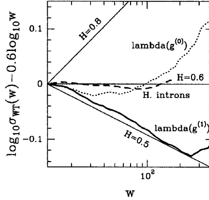
Figure 5. Scale-invariance analysis of the DNA sequence of the bacteriophage \lambda ( L = 48502 ) using the Purine coding: \log_{10} \sigma_{WT}(w) - 0.6 \log_{10} w vs \log_{10} w . \sigma_{WT}(w) corresponds to the variance of the wavelet coefficients computed at scales w (in bp units) with the zero-order g^{(0)} (smooth box: dotted line) and first-order g^{(1)} (the first derivative of the Gaussian function: solid line) analyzing wavelets illustrated in Figures 6(c) and 6(d) respectively. The results obtained for our set of human introns with g^{(1)} (dashed line) are shown for comparison. Note that when using g^{(0)} , \sigma_{WT}(w) actually corresponds to w\sigma_H(w) (see equations (2) and (8)).
