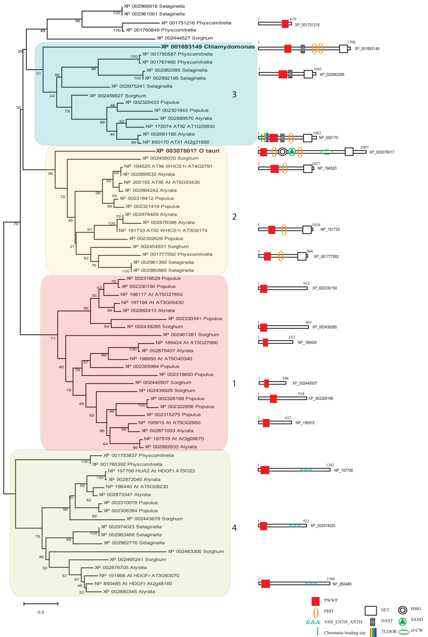
Additional File 8. Neighbor-Joining phylogeny of PWWP containing proteins in plants including the ATX3-like protein from O. tauri and the ATX1-like protein of Chlamydomonas . The tree was constructed as described in Additional file 5. Phylogenetic analyses were conducted in MEGA4.
