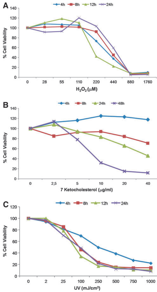
SUPPLEMENTARY FIG. S2. Loss of cell viability measured at indicated time points as a result of H 2 O 2 (A), 7-ketocholesterol (B), and UV (C) treatment. An average of triplicate experiments is shown in figure for normal cells versus patient cells. Cell viability is measured with WST-1 reagent (Roche).
