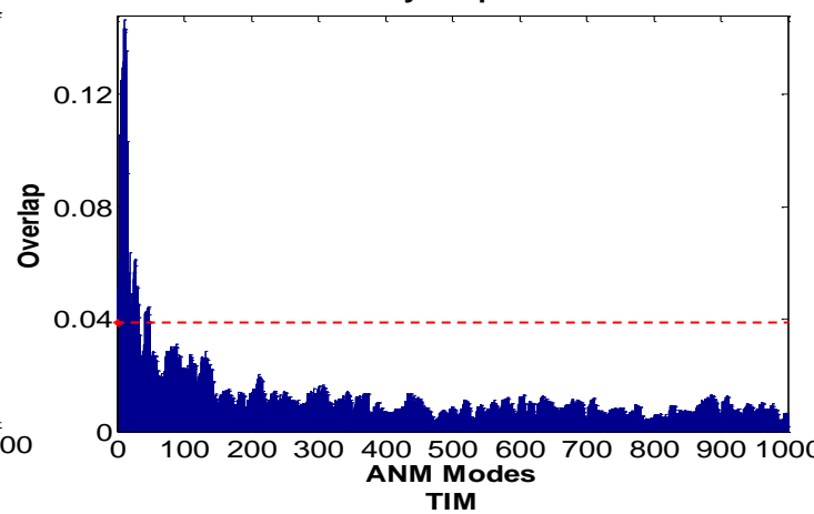
3-dehydroquinase
