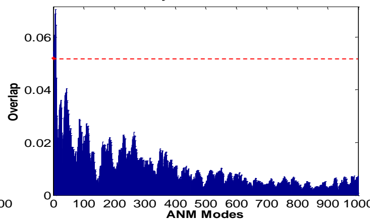
Pyruvate Mutase
