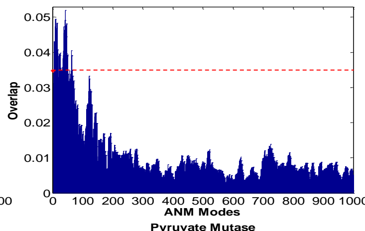
TIM
