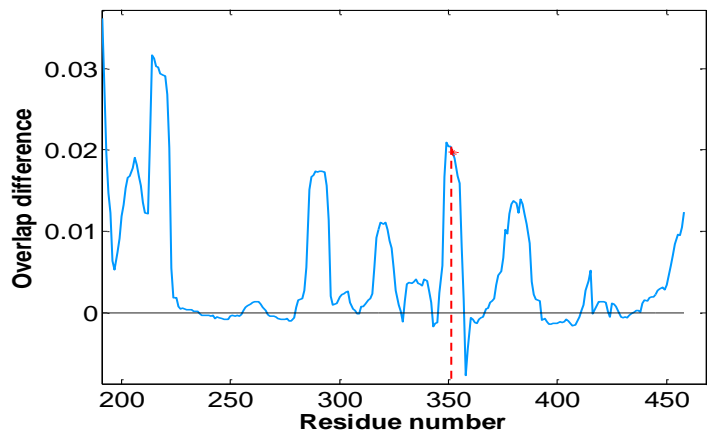
L-lactate dehydrogenase
