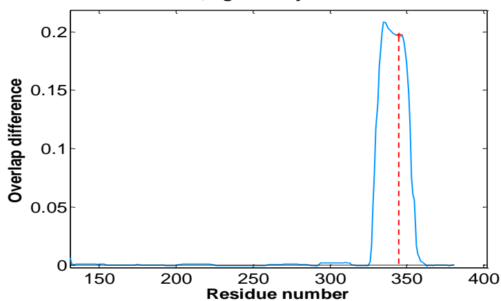
3-dehydroquinase
