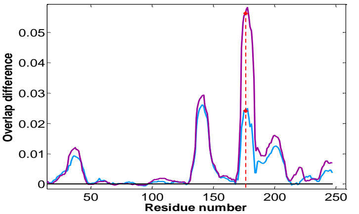
Pyruvate Mutase
