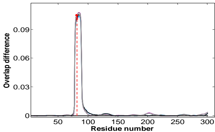
Biphosphate aldase
