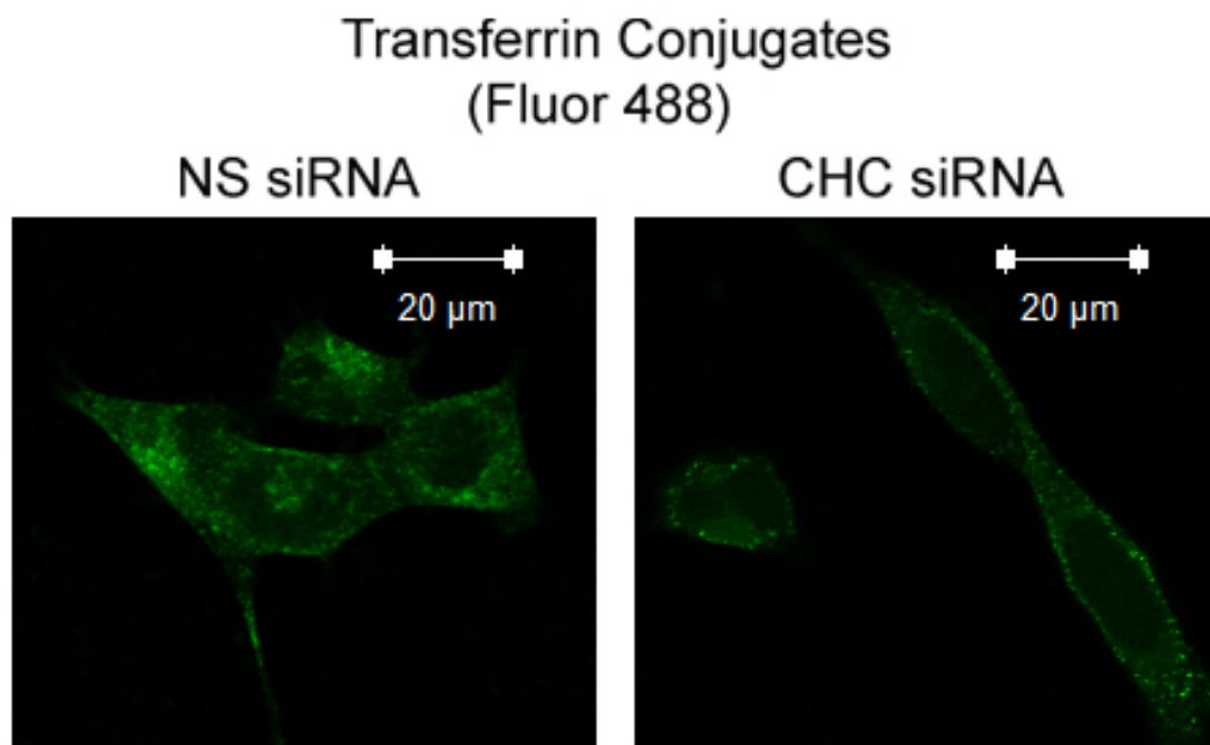
Figure S6 Depletion of clathrin heavy chain with siRNA effectively blocks clathrin-mediated endocytosis. HEK293 cells transfected with nonspecific or CHC siRNA were labeled by transferrin conjugated with Fluor 488 at 4 °C for 30 min and followed by incubation at 37 °C for 10 min. Images were visualized with confocal microscopy.
