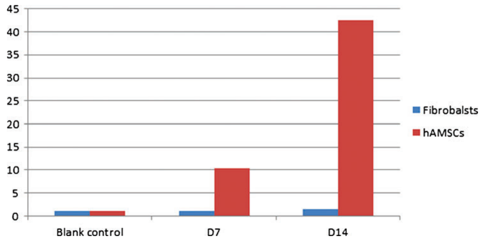
SUPPLEMENTARY FIG. S3. Real-time PCR of Oct4 expression in reprogrammed hAMSCs and fibroblasts. Real-time PCR results demonstrated a 20-fold increase in Oct4 expression in the hAMSCs compared with the fibroblasts by day 14.
