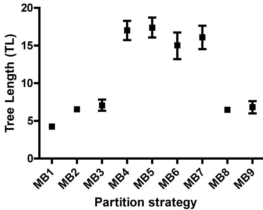
Supplementary Figure S4. Model partitioning increases the mean tree length (TL) and run variance. Shown is a box plot indicating the mean TL and 95% confidence interval among partitioning strategies.
