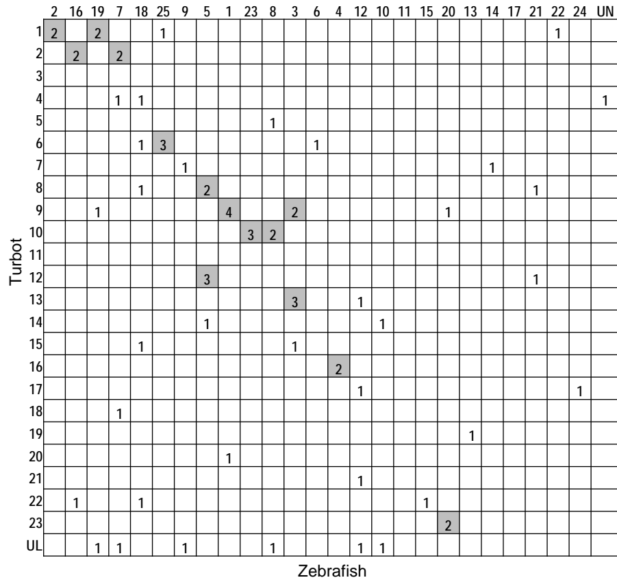
FIGURE S4. Oxford grid showing syntenies between the turbot linkage map and the zebrafish genome. In gray background syntenies with two or more significant hits. UL: unlinked markers in the turbot map; UN: unrandom genomic regions of the model fish species.
