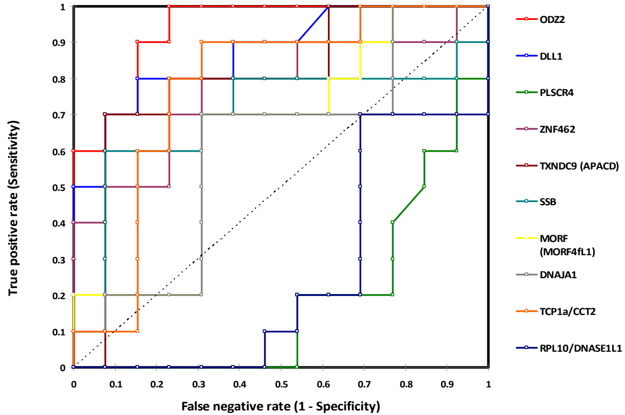
ROC Curves for Individual Genes in the Signature (MA Analysis)
