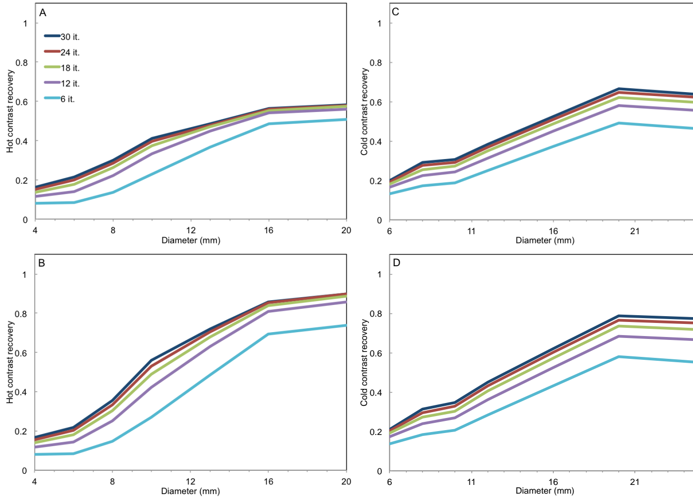
Supplementary Figure 7. Contrast recovery in function of the number of iterations for General Electric Discovery NM/CT670. Reconstructions were performed with General Electric Evolution for Bone including attenuation and scatter correction and resolution recovery and eight subsets. (A, B) Hot rods. (C, D) Cold rods. (A, C) Full ROI. (B, D) Half ROI.
