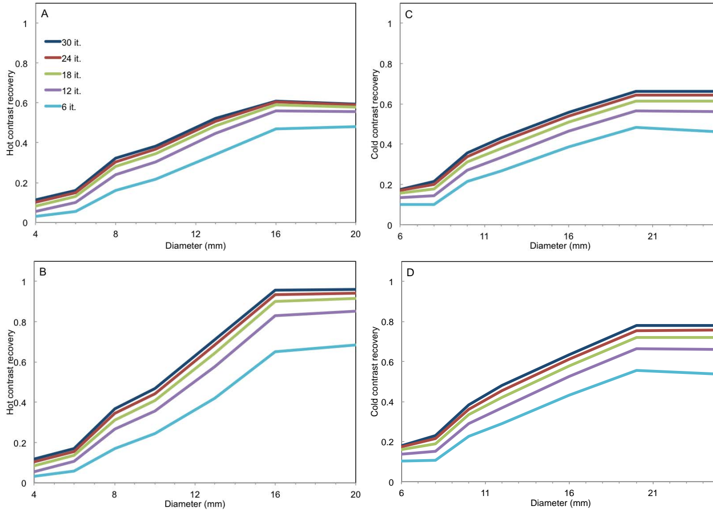
Supplementary Figure 9. Contrast recovery as a function of the number of iterations for the Siemens Symbia T6. Reconstructions were performed with Siemens Flash3D including attenuation and scatter correction and resolution recovery and eight subsets. (A, B) Hot rods. (C, D) Cold rods. (A, C) Full ROI. (B, D) Half ROI.
