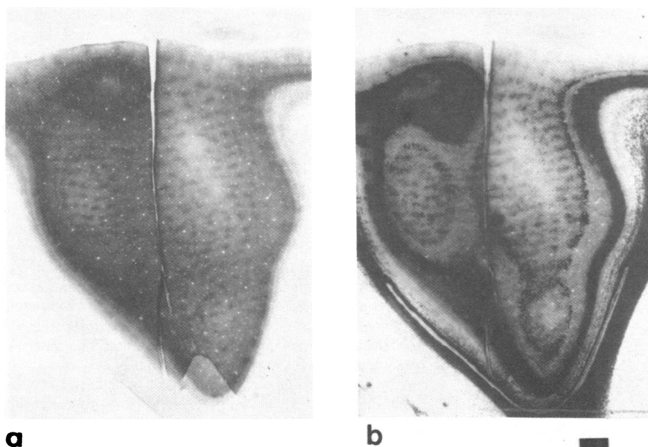
FIG. 1. (a) Cytochrome oxidase pattern in macaque monkey striate cortex. Films of two adjacent sections were overlaid by lining up radial blood vessels to accentuate the pattern. (b) Autoradiogram of two overlaid adjacent cortical sections. This monkey had been injected with 0.2 mCi of [ ^3\text{H} ]proline in the ipsilateral lateral geniculate nucleus. The photograph is a negative dark field, so the silver grains appear dark. Overlaying films of the cytochrome oxidase pattern and the autoradiograms shows that the two blob patterns are in register. These sections are tangent to buried cortex in the calcarine roof, so the upper layers are in the three coalescing central regions surrounded by deeper layers. Bar = 1 mm.
